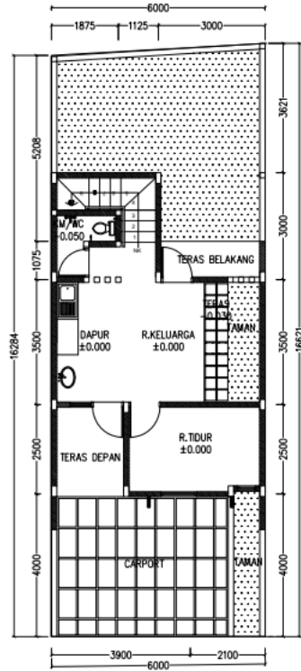
DENAH LANTAI DASAR
